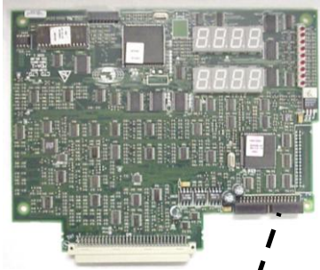
(11) MDA1 CPU 9200-0784
