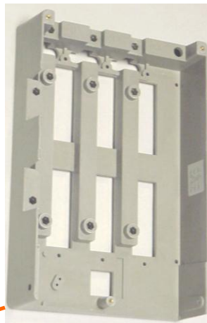
(6) Base P/N 3810-0016
