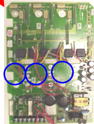
(24) MDA210 P/N 9200-0619
